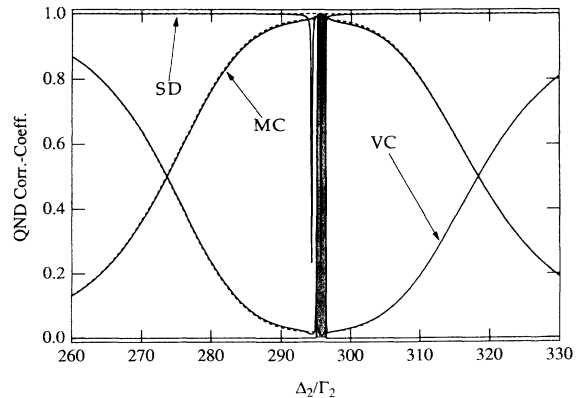
FIG. 8. Zero-frequency correlation coefficients for the ladder scheme vs scaled atom-probe detuning \Delta_2/\Gamma_2 . The parameters are the same as in Fig. 4 except that the decay rate of the upper transition is decreased by a factor of 4. The dashed lines represent the analytical approximated result. The gray area is the unstable region.
