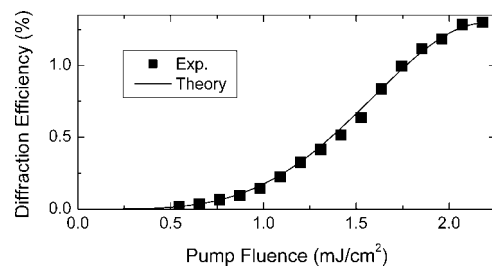
Fig. 3. Diffraction efficiency versus write fluence.
