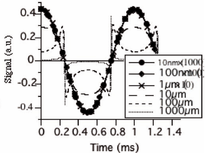
Figure 4 : Numerical simulation of the velocimeter response, for a sinusoidal displacement at 1kHz. The curves at the lowest amplitudes (0.01µm to 1µm) are compensated for their amplitude. They superpose exactly showing the linearity of the response of the velocimeter.
